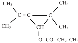
2 : 2 - Dimethyl - 3 - isopropylidene - cyclopropyl Propionate
